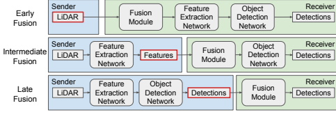
Figure 1: Taxonomy of cooperative perception systems.
