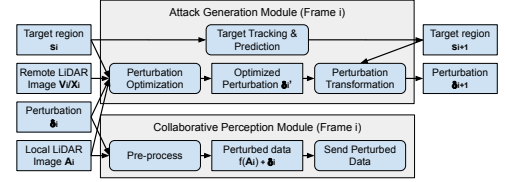
Figure 3: Framework of real-time targeted attacks on collaborative perception.
